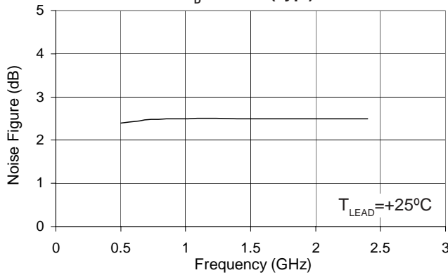
Noise Figure vs. Frequency I D = 35 mA (Typ.)
