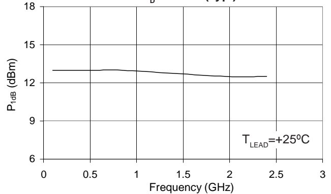
P 1dB vs. Frequency I D = 35 mA (Typ.)
