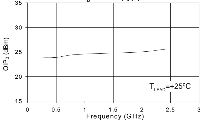
OIP 3 vs. Frequency I D = 35 mA (Typ.)
